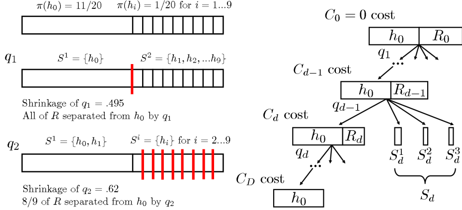
Fig. 1. Left: Counter example showing that when a single hypothesis h_0 contains more than half the mass, the query with maximum shrinkage is not necessarily the query that separates the most mass from h_0 . Right: Notation for this case.
