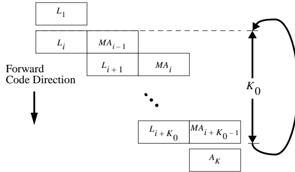
Figure 6: Two stage software pipelining.
