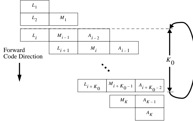
Figure 5: Three stage software pipelining. The loads for the first two loop iterations and the multiplies for the first iteration are factored out of the unrolled inner-most loop as are the multiplies for the penultimate and the accumulates for the last two loop iterations.
